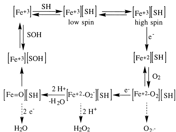
Figure 1. Catalytic cycle of cytochrome P450, showing the individual steps at which uncoupling can occur. The iron of the heme group is indicated as an iron atom in brackets.
