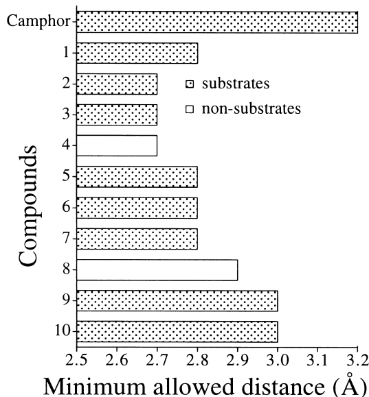
Figure 3. Relationship between the minimum distance allowed to separate a substrate and a protein atom and the prediction by DOCK that the compound is a substrate. The solid bars indicate compounds shown experimentally to be substrates, and the open bars compounds shown not to be substrates. The bars end at the minimum allowed distance beyond which the compounds are predicted by DOCK to not be substrates. The enzyme used in this study was wild-type ferric P450 cam .
