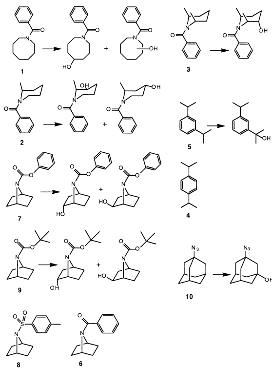
Figure 2. Structures of the compounds tested as potential substrates for P450 cam and of the metabolites obtained from them.
